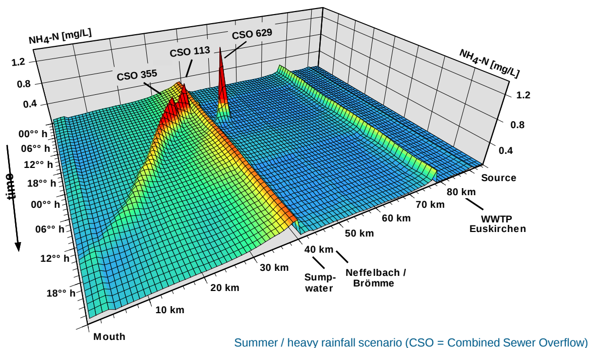
Figure 1: Ammonium concentration during heavy precipitation in the middle reaches of the Erft (model coupling: NASIM, LWA-FLUT and DWA Water Quality Model; CSO = combined sewer overflow, GWK = collective wastewater treatment plant)
